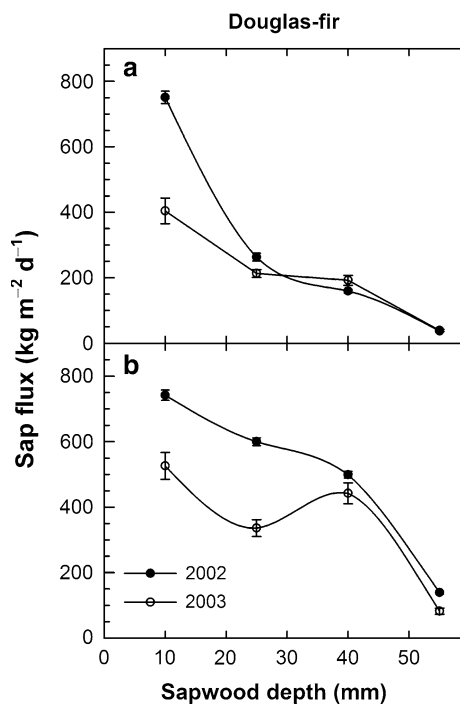
Fig. 4 Radial profiles of mean daily total sap flux in two large Douglas-fir trees (see a and b ) for six comparable paired days in August 2002 and 2003. Mean daytime vapor pressure deficit ( \delta ) was 1.74 (0.17) and 1.77 (0.09) kPa, mean daytime photosynthetic photon flux was 923 (20) and 861 (26) \mu\text{mol m}^{-2} \text{s}^{-1} , and mean daily soil volumetric water content at 60 cm was 21% (0.4) and 21.8% (0.9) in 2002 and 2003, respectively. Standard errors denoted in parentheses above and in the figure are based on n = 6 days
